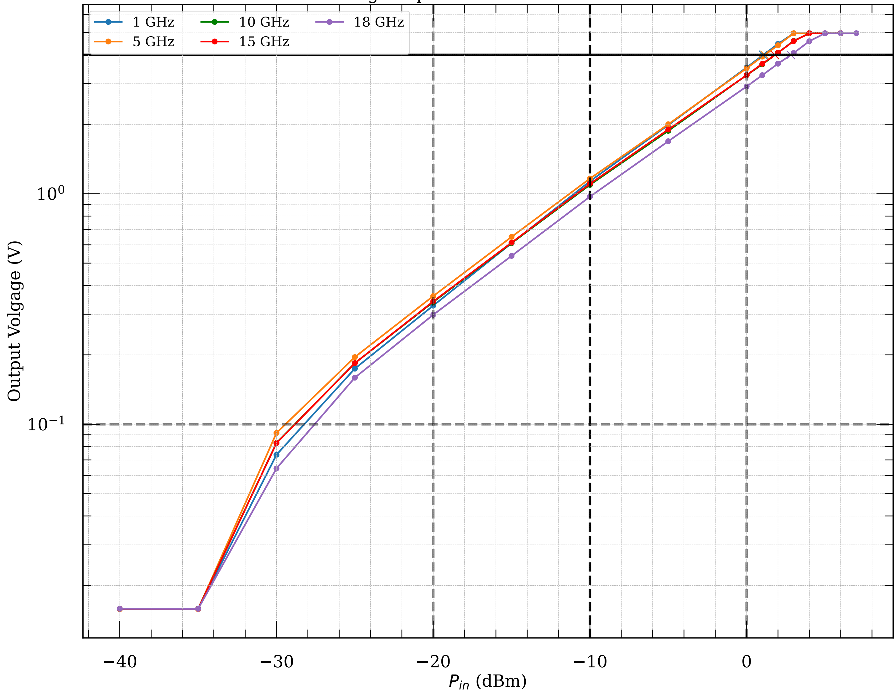
Measured voltage-to-power curve of detector module087v2
